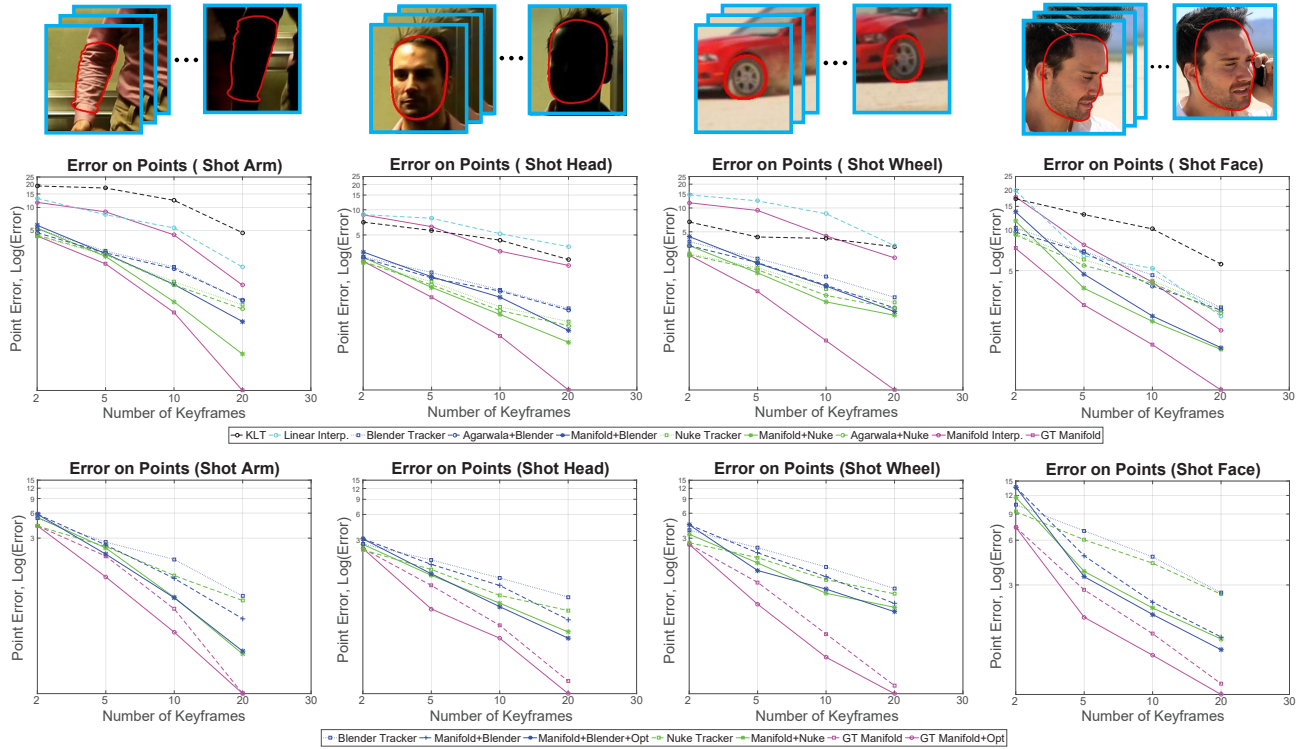
Figure 7: Quantitative evaluations on selected shots of our Real-World Rotoscoping Dataset. The First Row (from left to right) shows the shots i.e. Arm , Head , Wheel and Face that represent several typical objects and motions. The Second Row shows the evaluation on the selected shots by using various interpolation methods, i.e. our Manifold with either Ground Truth tracking (“GT”), Nuke Planar Tracker or Blender Planar Tracker; the regularization of Agarwala et al. [2004]; the KLT Tracker; and Linear Interpolation. The Third Row illustrates the performance improvement on our manifold methods using optimal keyframe selection (for methods marked with “+OPT”). Errors (shown on log plots) are calculated using the RMS pixel error between the control points of estimated curves and the ground truth (both have the same parameterization).
